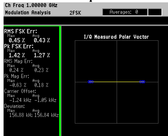
Figure 2-22 I/Q Measured Polar Graph
