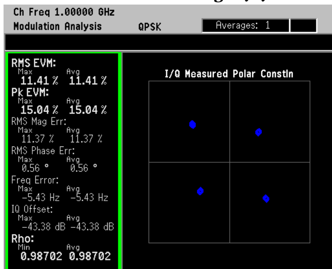
Figure 2-56 Polar Constellation Showing I/Q Quadrature Skew
