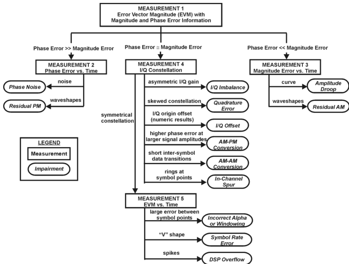
Figure 2-48 Flow Chart for EVM Troubleshooting
