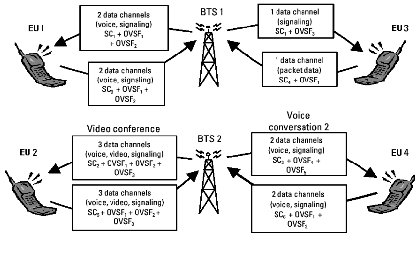
Figure 4-63 W-CDMA Code Allocations
