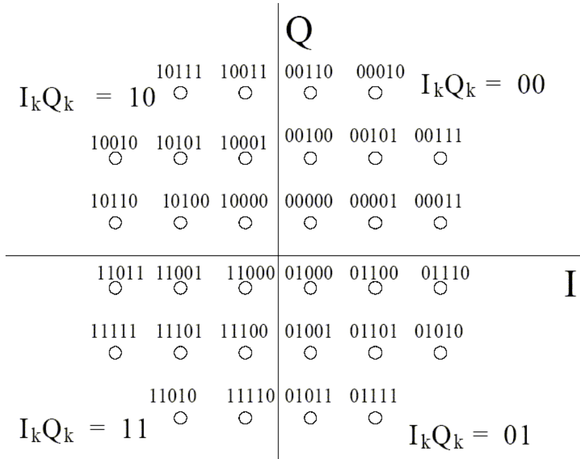
Figure 4-56 DVB 32QAM Bit State Diagram
